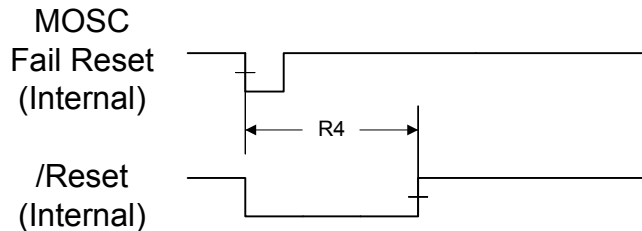
Figure 20-10. MOSC Failure Reset Timing
