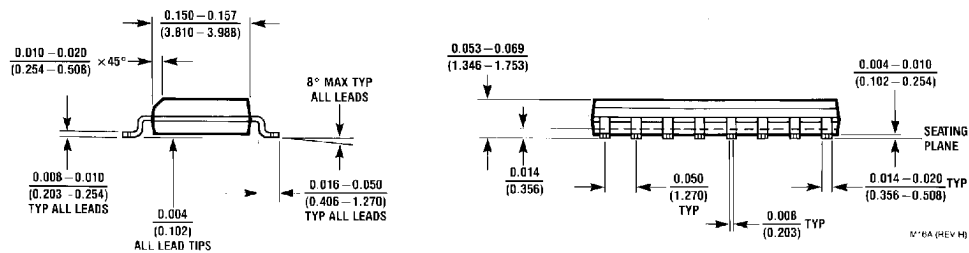
16-Lead Small Outline Molded Package (M) Order Number DM74LS190M, DM74LS191M NS Package Number M16A
