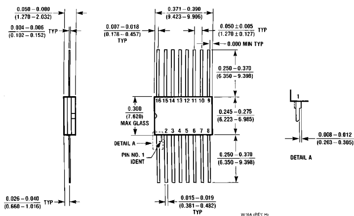
16-Lead Ceramic Flat Package (W) Order Number DM54LS190W or DM54LS191W NS Package Number W16A
