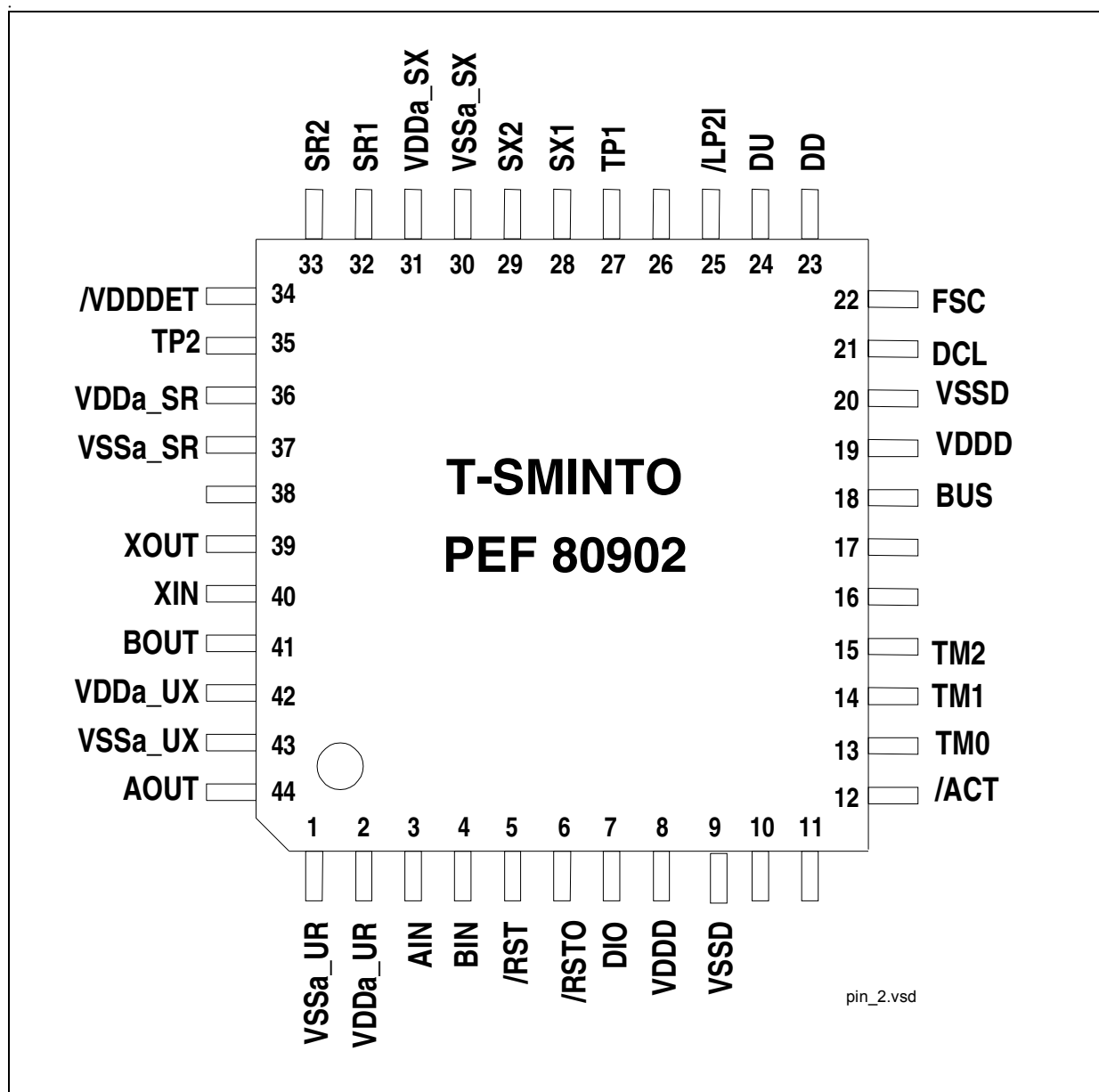
Figure 1 Pin Configuration
