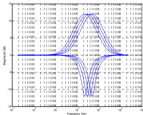
Figure 44 EQ Band 2 – Peak Filter Centre Frequencies, EQ2BW=0
