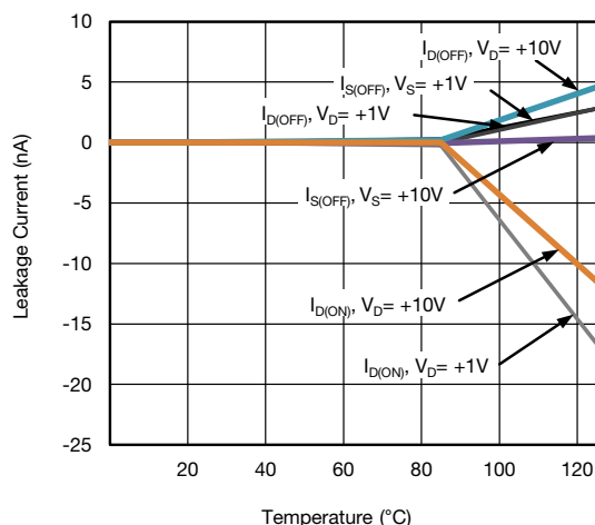
Leakage Current vs. Temperature ( +12\text{ V} )
