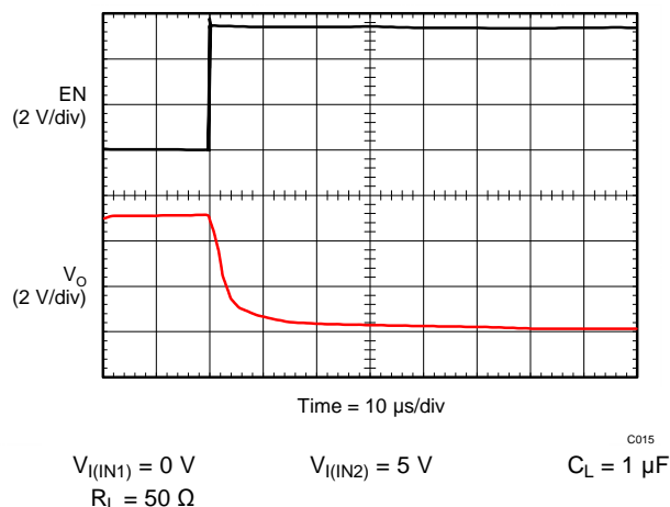
Figure 18. Propagation Delay and Fall Time With 1- \mu F Load, IN2 Turnoff
