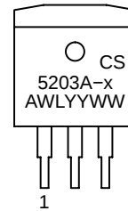
D 2 PAK-3 DPS SUFFIX CASE 418F
