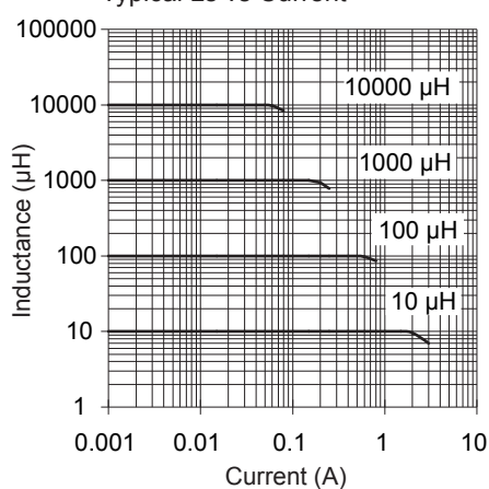
Typical Ls vs Current
