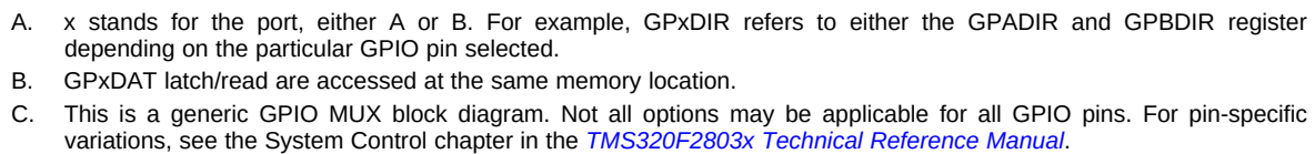
Figure 6-45. GPIO Multiplexing
