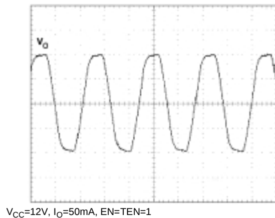
Figure 25 : 22kHz Tone Waveform
