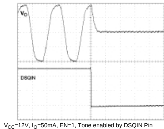
Figure 28 : DSQIN Tone Disable Transient Response
