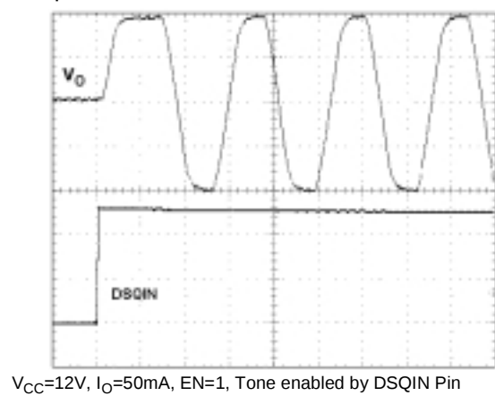
Figure 26 : DSQIN Tone Enable Transient Response
