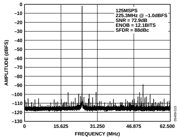
Figure 15. AD9445-125 64k Point Single-Tone FFT/125 MSPS/225.3 MHz
