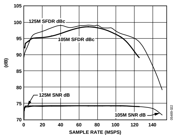
Figure 22. AD9445 Single-Tone SNR/SFDR vs. Sample Rate 2.3 MHz
