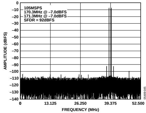
Figure 43. AD9445-105 64k Point Two-Tone FFT/105 MSPS/170.3 MHz, 171.3 MHz
