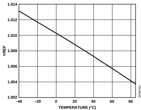
Figure 49. AD9445-125 VREF vs. Temperature
