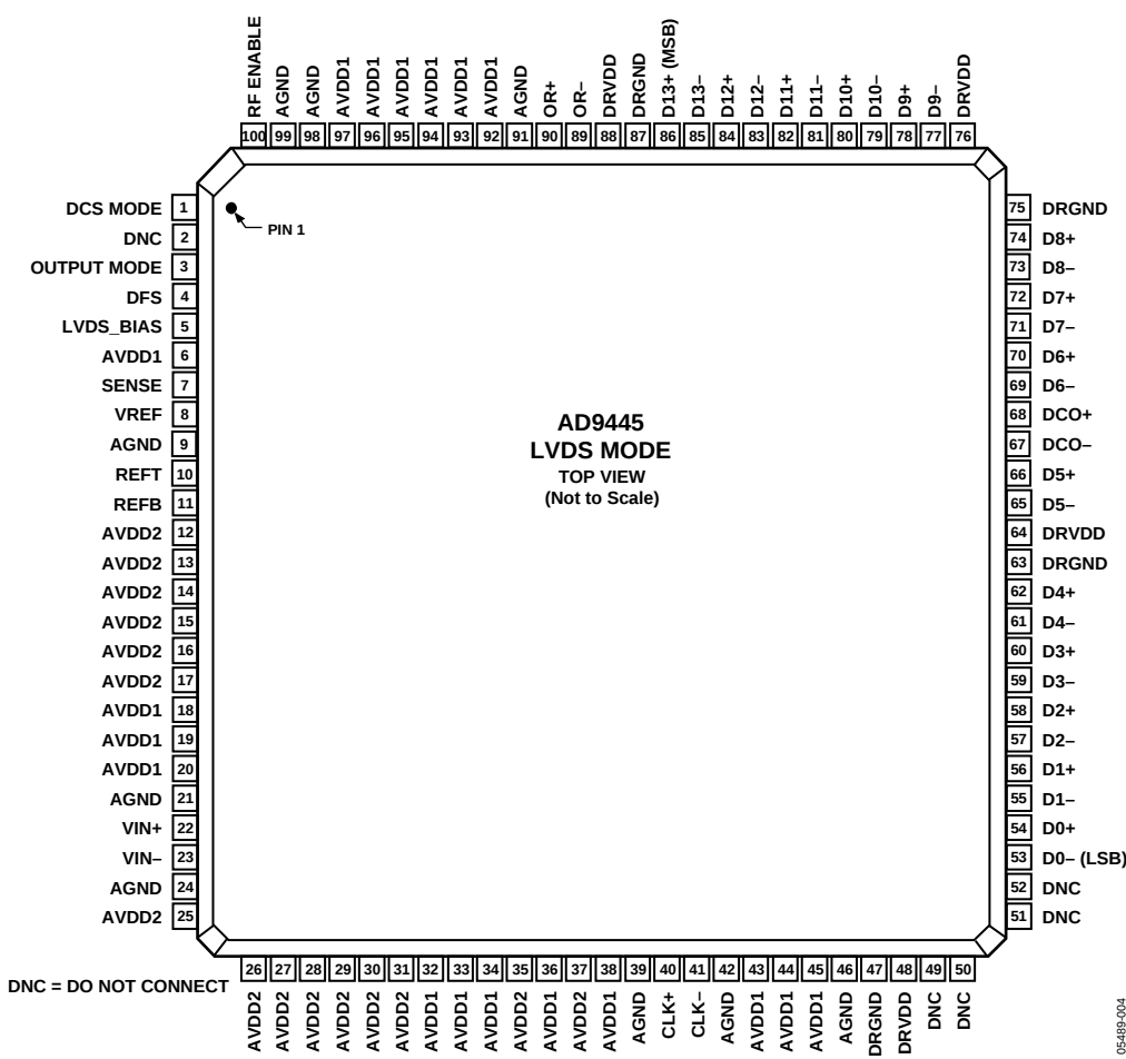
Figure 4. 100-Lead TQFP/EP Pin Configuration in LVDS Mode
