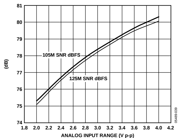
Figure 58. SNR vs. Analog Input Range, 2.3 MHz @ -30 dBFS
