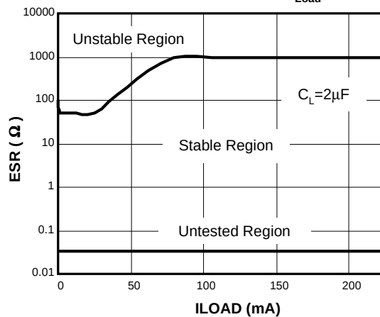
Stability vs. ESR vs. I_{Load}
