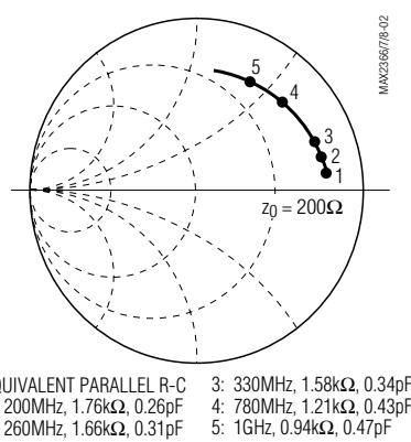
TANK 1/S11 vs. FREQUENCY
