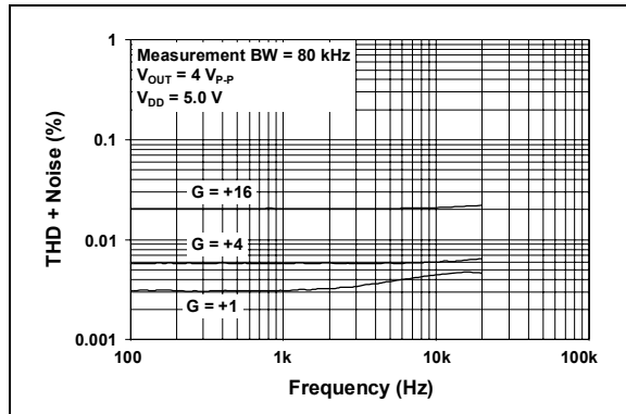
FIGURE 2-28: THD plus Noise vs. Frequency, V_{OUT} = 4 V_{P-P}
