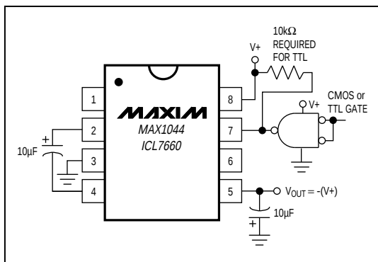
Figure 7. External Clocking
