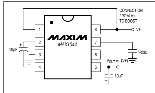
Figure 6. Negative Voltage Converter with C_{OSC} and BOOST
