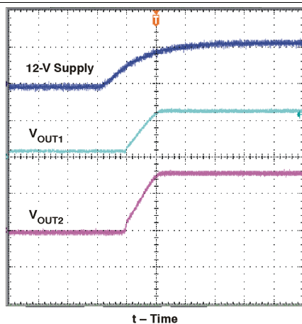
Figure 22. Start-Up Waveforms
