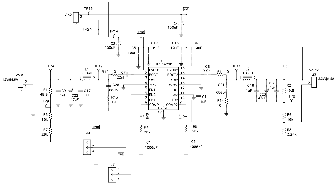
Figure 21. Cascading Operation
