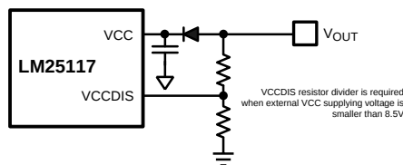
Figure 16. External VCC Supply For 5 V < V_{OUT} < 14.5 V
