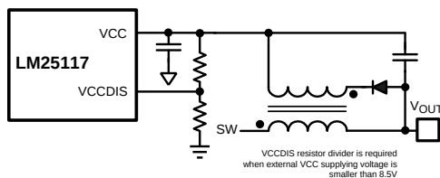
Figure 17. External VCC Supply For V_{OUT} < 5 V
