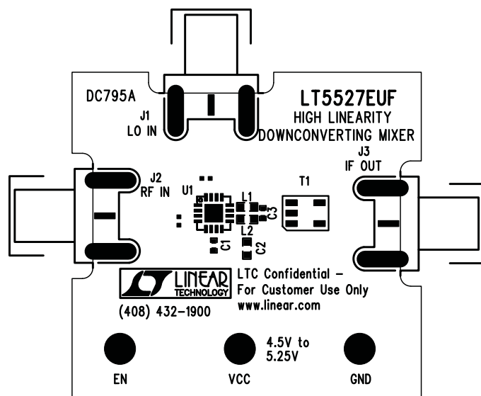
Standard Evaluation Board Layout
