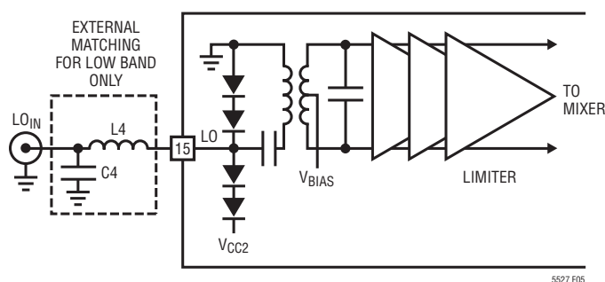
Figure 5. LO Input Schematic
