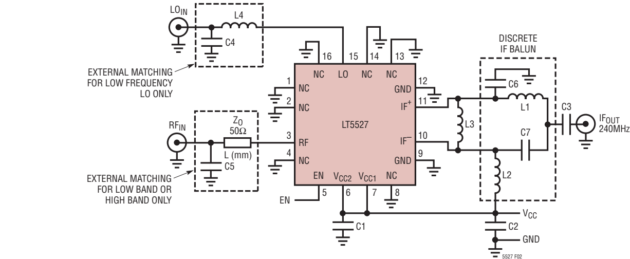
Figure 1. Downmixer Test Schematic—Standard IF Matching (240MHz IF)
