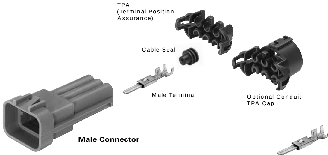
2.8 Male Connector Sealed
