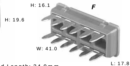
12176478 Cap Assembly 4-3M Mates to Connector 12176473
