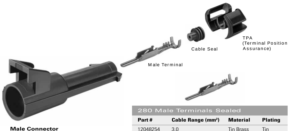
Male Connector
