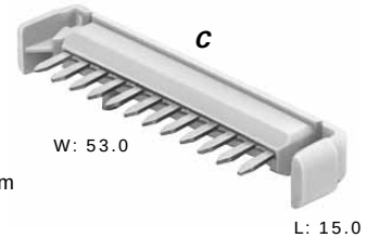
12176469 Cap Assembly 2-6M Mates to Connector 12176460
