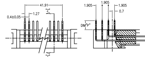
VIEW "Y"-Y"(4/1)
