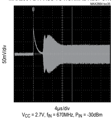
MAX2664 BYPASS TO NORMAL RESPONSE
