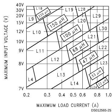
FIGURE 5. LM2595-5.0
