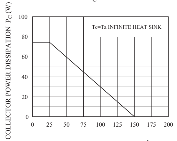
AMBIENT TEMPERATURE T_a ( ^{\circ}C )
