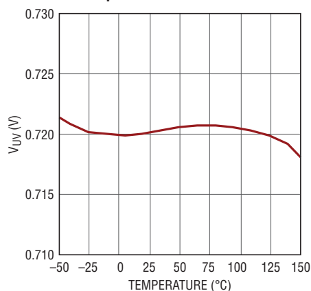
Power-On Reset Threshold vs Temperature
