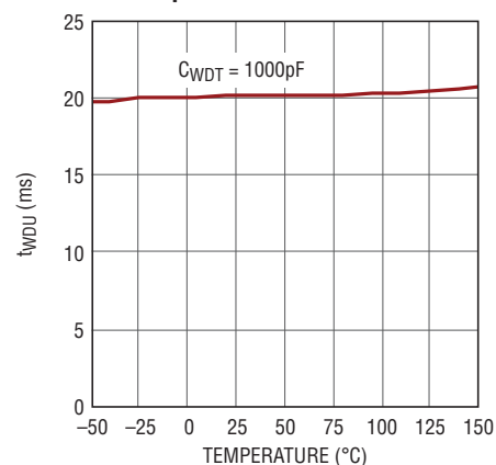
Watchdog Window Mode Period vs Temperature
