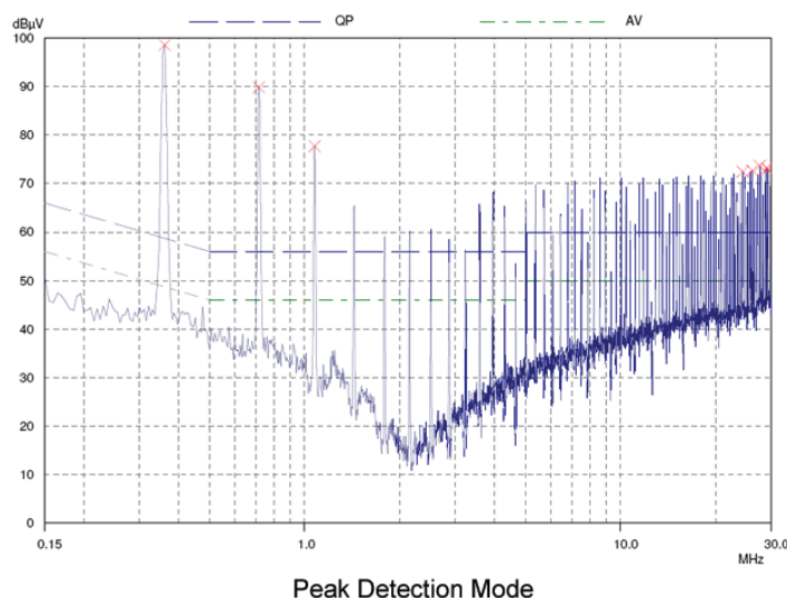
Graph 1. Conducted emissions performance, CISPR/EN55022, Class B, full load, unfiltered
