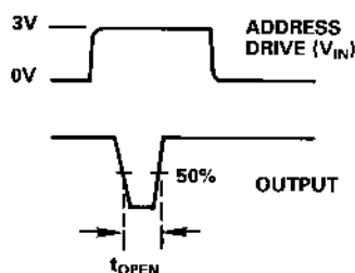
Test Circuit 7. Break-Before-Make Delay, t_{OPEN}
