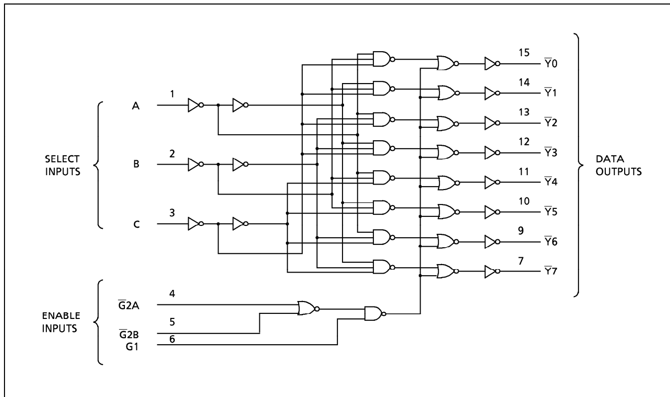
LOGIC DIAGRAM
