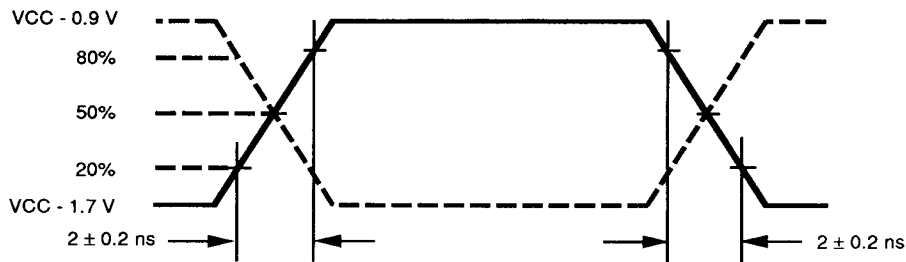
ECL Input Waveform
