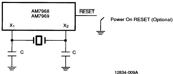
Figure 1. Connections for 12.5-17.5 MHz
