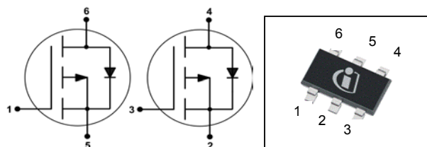
PG-TSOP6
