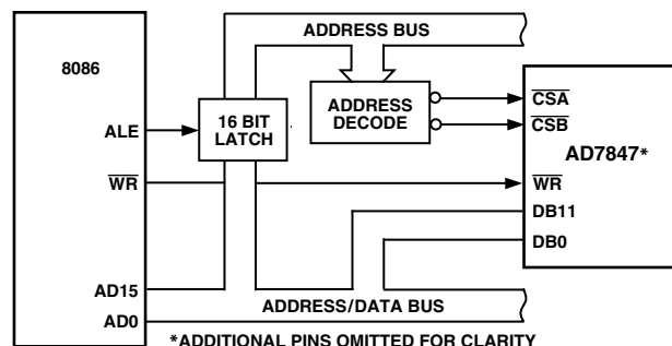
Figure 20. AD7847 to 8086 Interface
