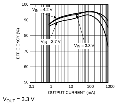
Figure 39. Autmode Efficiency vs I_{LOAD}
