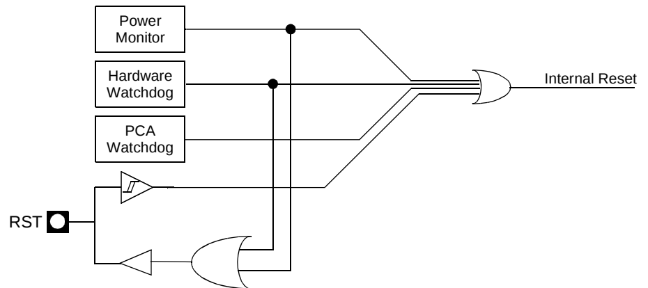
Figure 16. Reset Schematic
