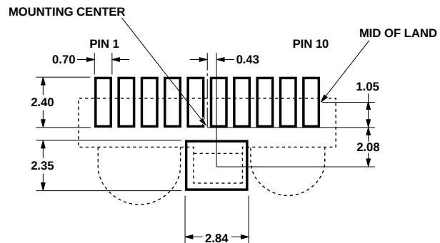
LAND PATTERN
