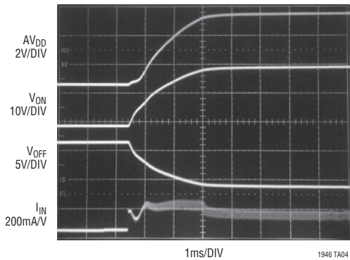
Start-Up Waveforms
