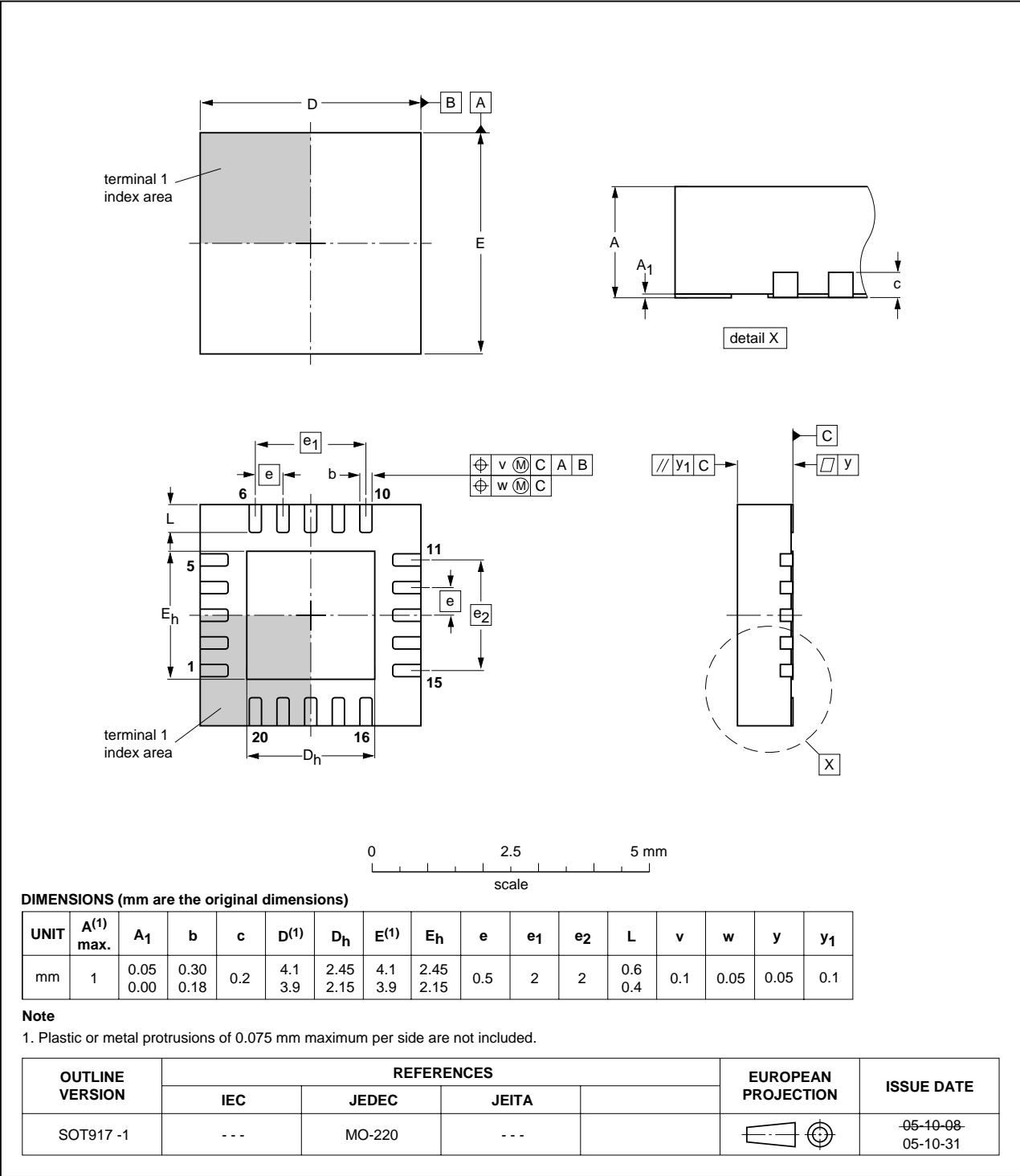
Fig 17. Package outline SOT917-1 (HVQFN20)
