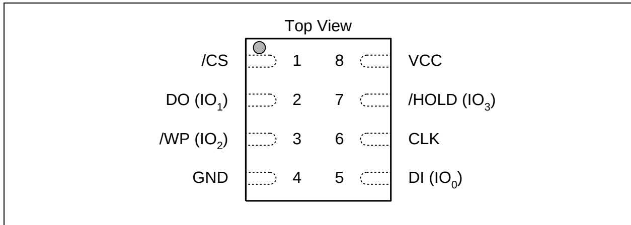
Figure 1b. W25Q16DV Pad Assignments, 8-pad WSON 6x5-mm / USON 4x3-mm (Package Code ZP,UU)
