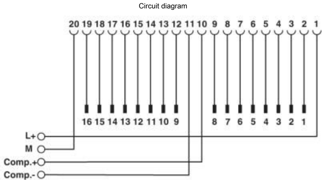
FLKM 16-PA-S300/MINI-MCR connection scheme
