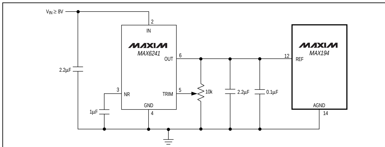
Figure 11. High-Accuracy Reference
