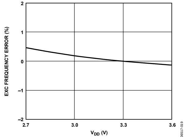
Figure 19. EXC Frequency Error vs. V_{DD}
