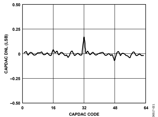
Figure 21. CAPDAC Differential Nonlinearity (DNL), V_{DD} = 3.3 V
