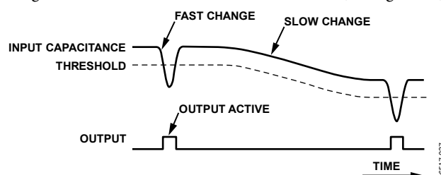
Figure 29. Adaptive Threshold Indicates Fast Changes and Eliminates Slow Changes in Input Capacitance
