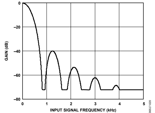
Figure 20. Capacitance Channel Frequency Response
