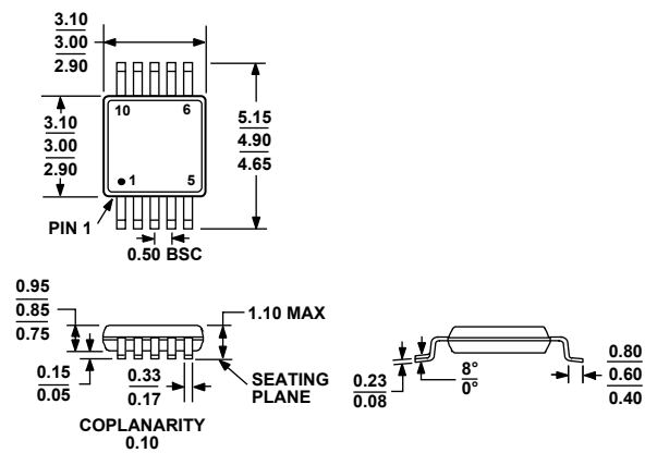
COMPLIANT TO JEDEC STANDARDS MO-187-BA Figure 54. 10-Lead Mini Small Outline Package [MSOP] (RM-10) Dimensions shown in millimeters
