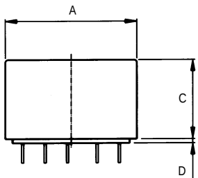
Housing A6
