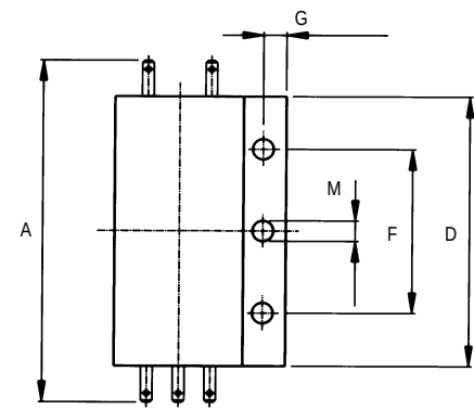
Housing A7B
