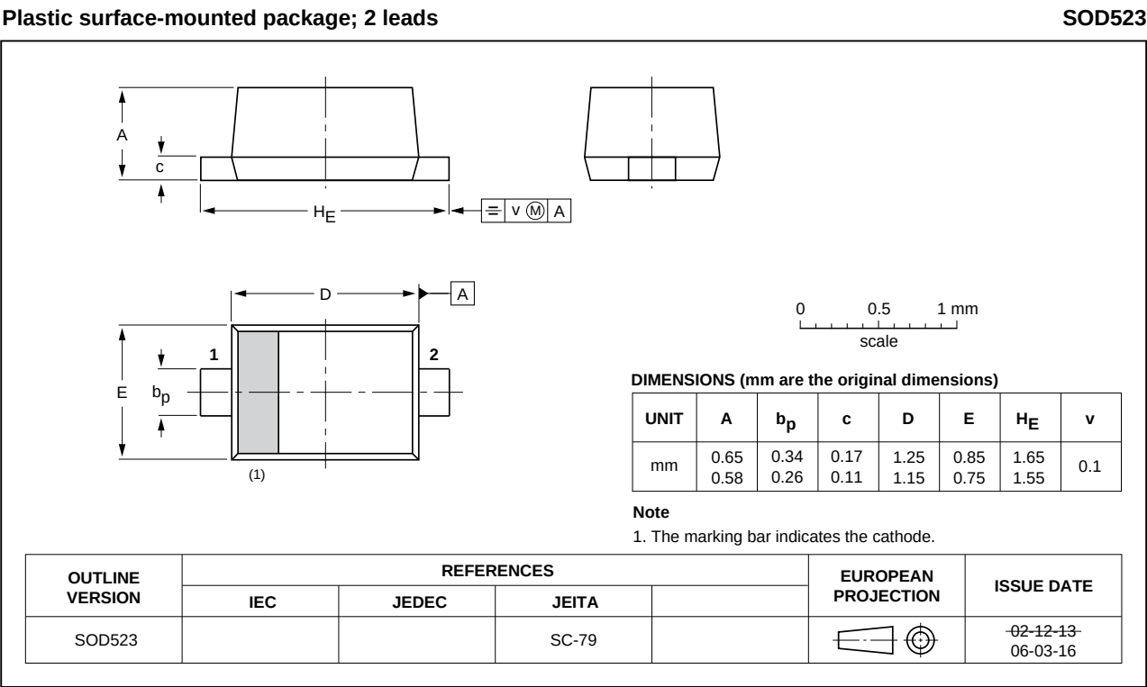
Fig 4. Package outline.
