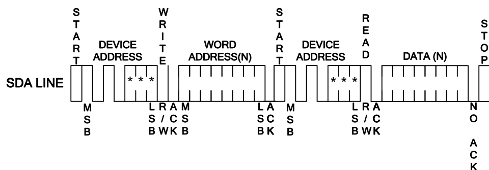
Figure 9: Random Read
