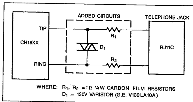
Figure 5. Additional Circuitry Needed for Canadian DOC Registration
