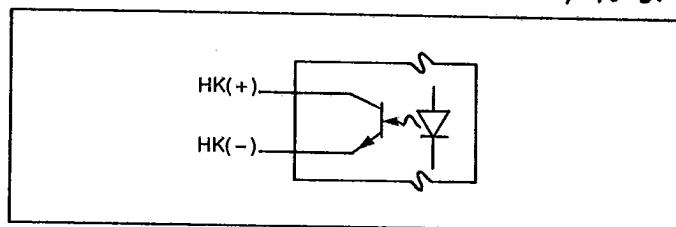
Figure 4. Hook Switch Detection Equivalent Output Circuit
