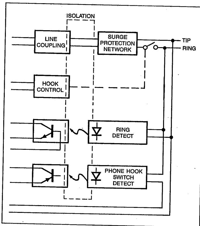
Figure 1. DAA Block Diagram
