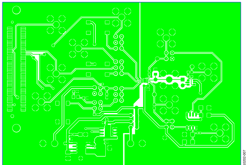
Figure 6. Component Side PCB Drawing
