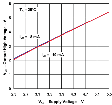
Figure 13. Output High Voltage vs Supply Voltage
