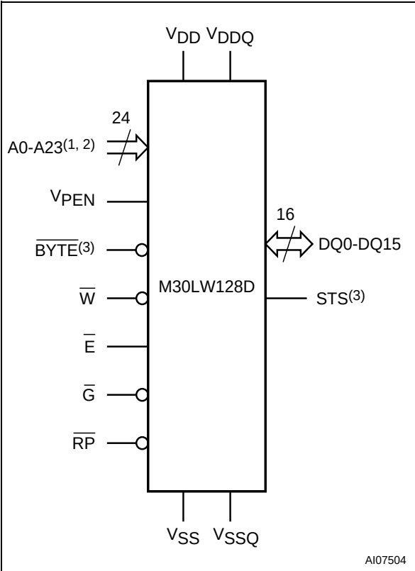
Figure 2. Logic Diagram
