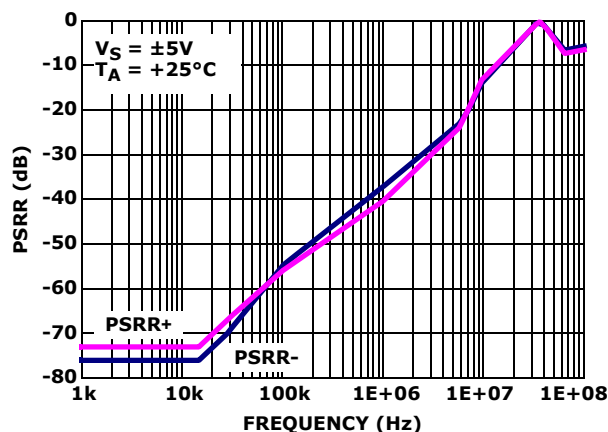
FIGURE 24. PSRR
