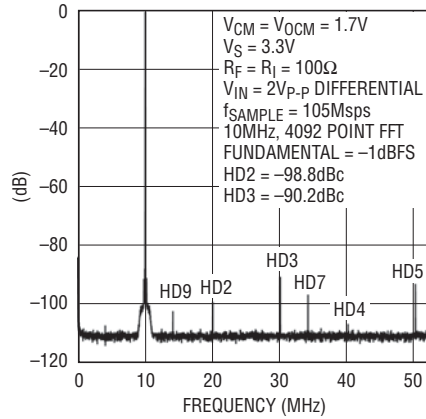
LTC6404-1 Driving LTC2207 16-Bit ADC
