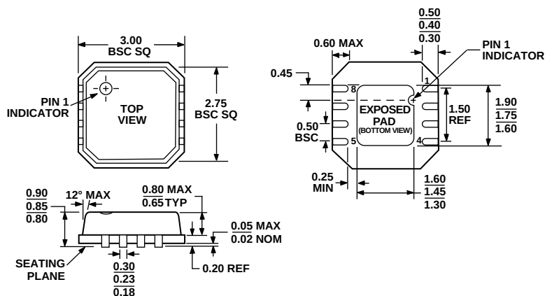
Figure 71. 8-Lead Lead Frame Chip Scale Package [LFCSP] 3 mm x 3 mm Body (CP-8-2)—Dimensions shown in millimeters
