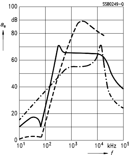
B84112-B-*60
