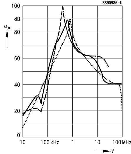
B84143-A120-R ... B84143-A180-R
